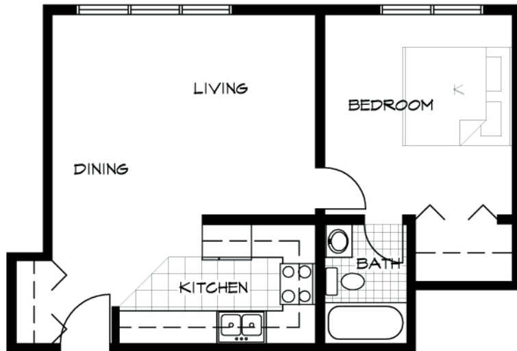
FLOOR PLAN - TYPICAL 1 BEDROOM 1/8" = 1'-0"
